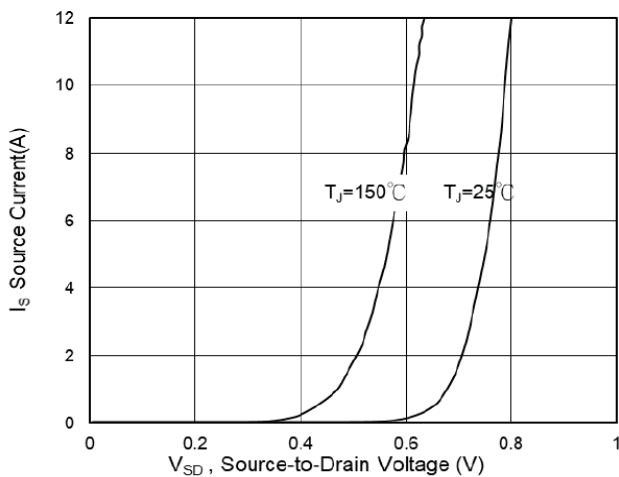
Figure 3: Source Drain Forward Characteristics
